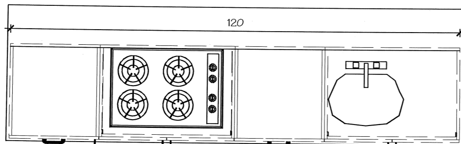
PLAN C108 HOME ECONOMICS SCALE = 1/2" = 1' - 0" ARCH REF A4.102
