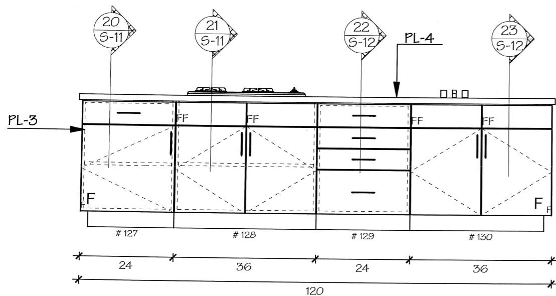
A ELEVATION C108 HOME ECONOMICS ISLAND SCALE = 1/2" = 1' - 0" ARCH REF 9/A4.102
